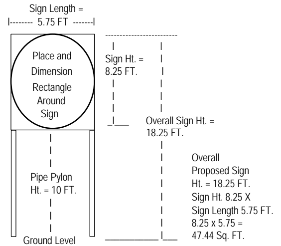
Freestanding Sign Elevation Detail #2
