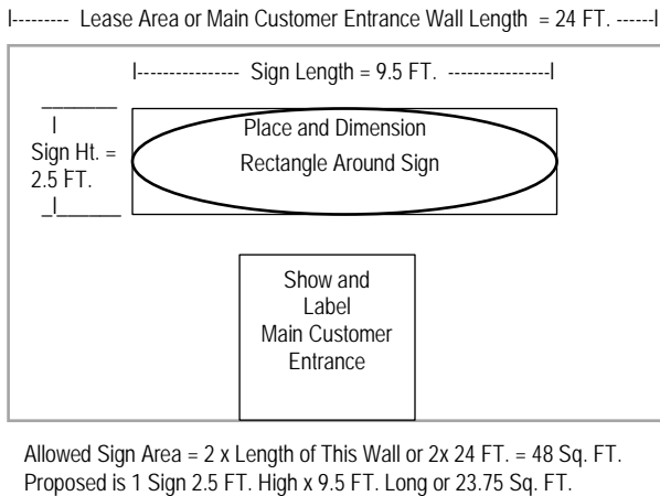
Wall Mounted Sign Elevation Detail #1
